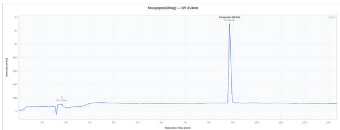
Kisspeptin 10mg - Lot-2026-05-28: UV Chromatogram
