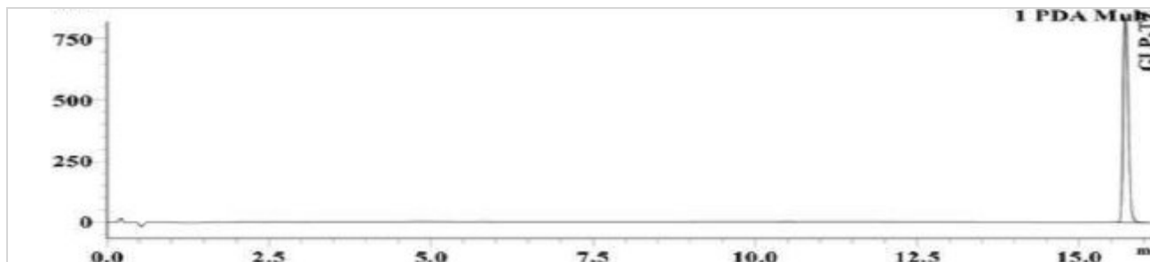
SPS-2TZ 10mg / GLP TZ - ABL-TIR-2602: UV Chromatogram
