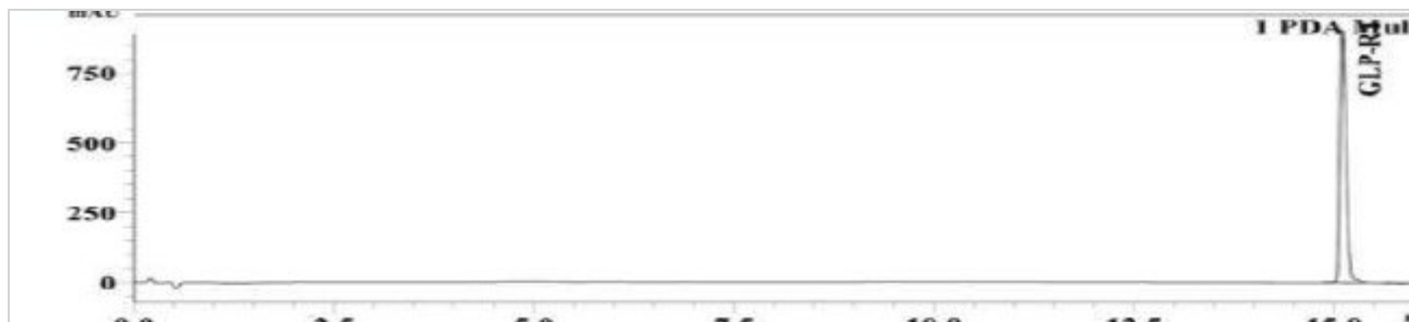
SPS-3RT 20mg / GLP RT - ABL-RET-2604: UV Chromatogram
