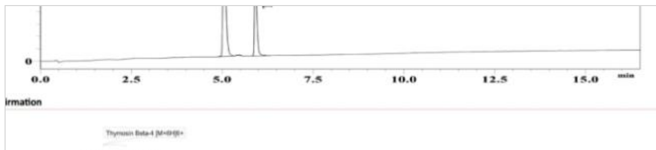
BPC-157 TB-500 10/10mg - ABL-RST-2602: UV Chromatogram
